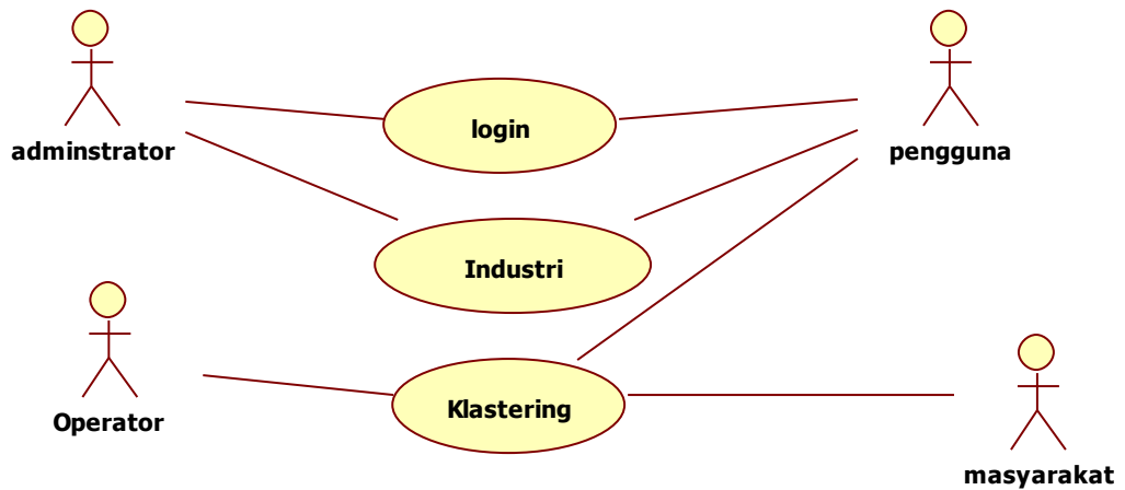
Gambar 1: Usecase Diagram
