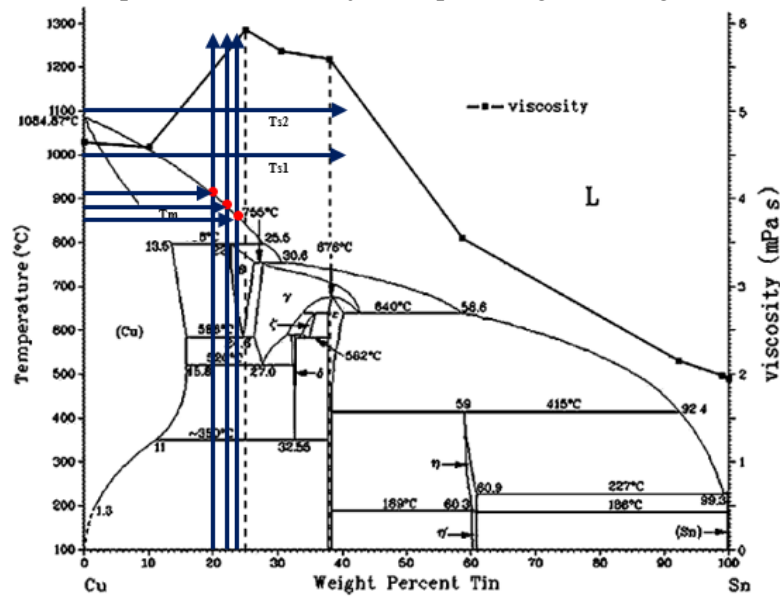
Gambar 2. Diagram fase Cu-Sn: Tm; Ts1=1000°C; Ts2=1100°C
