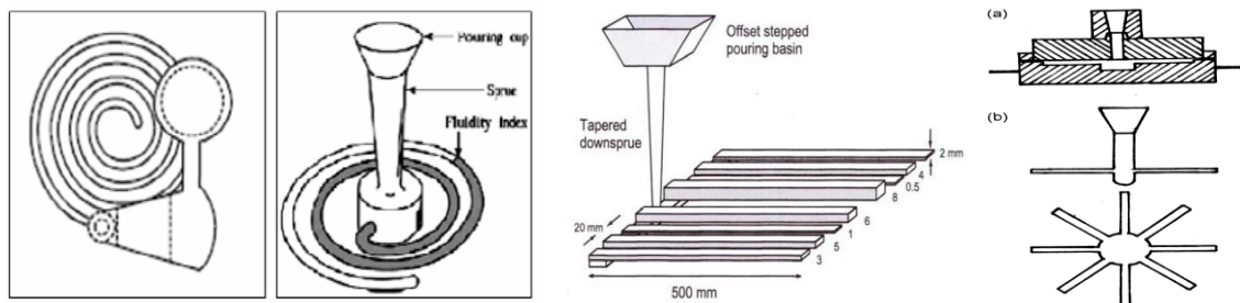
Gambar 1. (a) metode spiral (b) metode Birmingham, UK (c) metode Qudong
