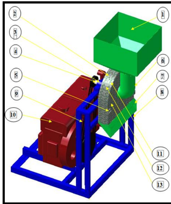
Gambar 7. Mesin hammer mill
