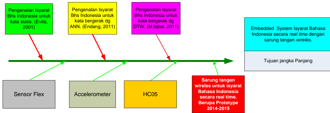
Gambar 4. Roadmap penelitian
