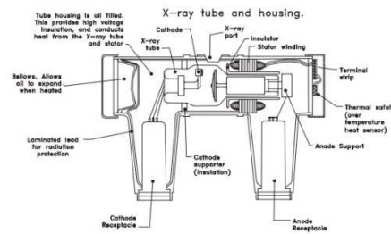
Gambar 2. Tabung Sinar-X dan Housing [Nasotih, 2015]
