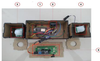
Gambar 3. Modul Sistem Monitoring
