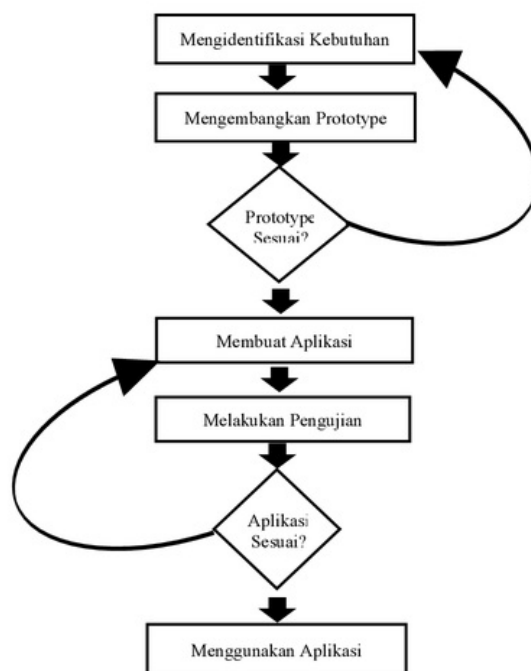
Gambar 3. Metode Prototyping
