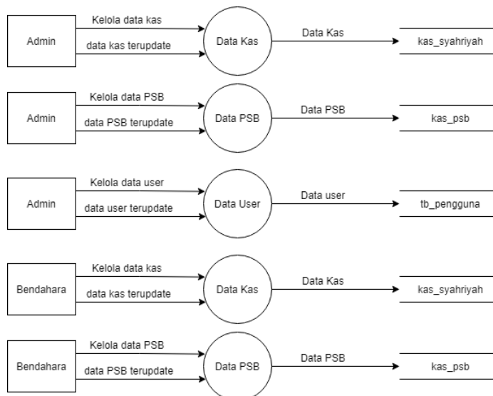
Gambar 5. DFD Level 2 (Data Flow Diagram)
