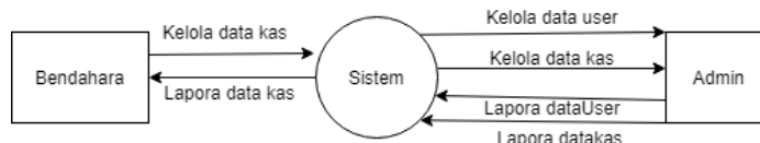
Gambar 3. DFD Level 0 (Data Flow Diagram)
