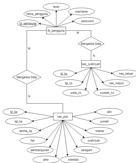
Gambar 2. ERD (Entity Relationship Diagram)
