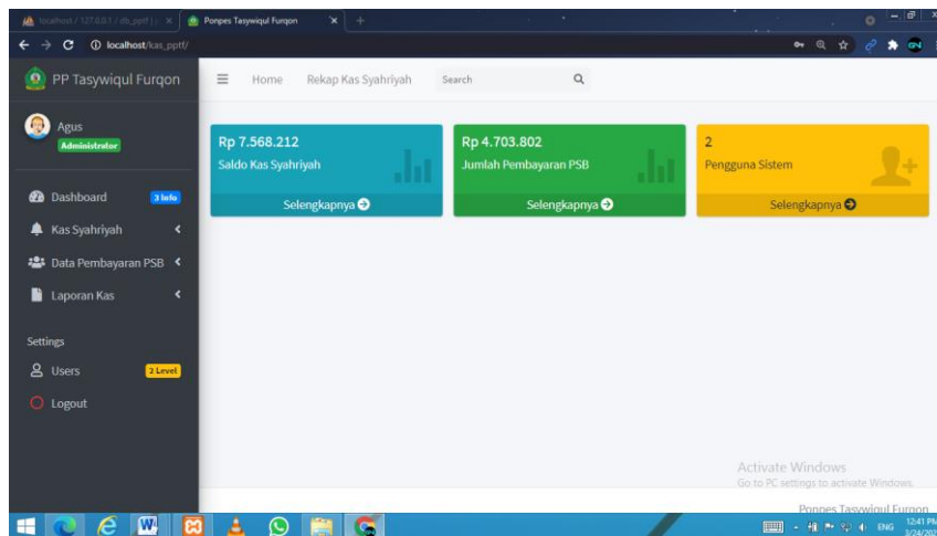
Gambar 7. Halaman Dashboard
