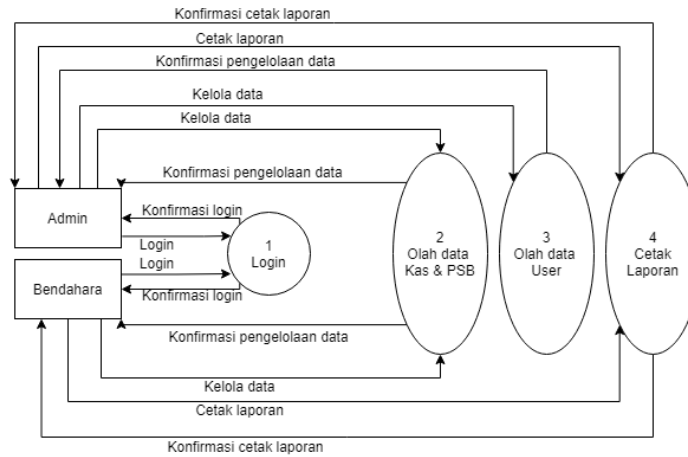
Gambar 4. DFD Level 1 (Data Flow Diagram)
